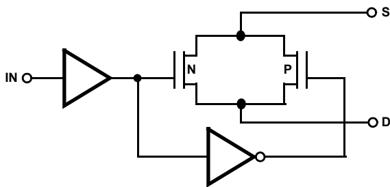
FIGURE 1. LOGIC CIRCUIT
